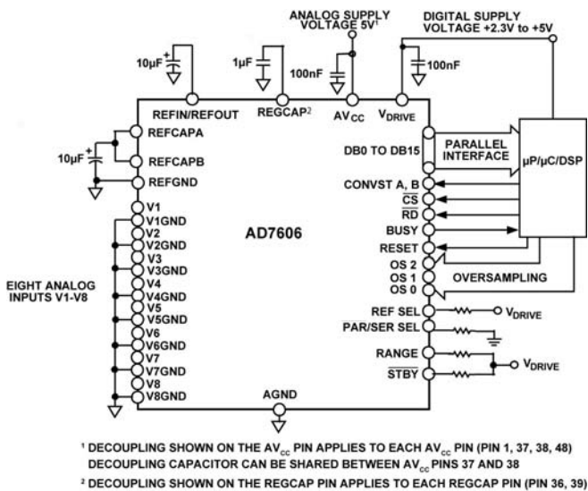
Figure 41 AD7606 Typical Connection Diagram
