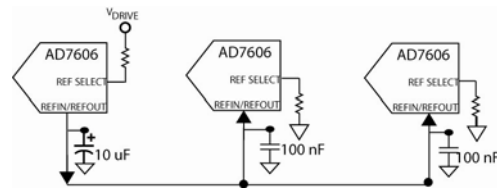
Figure 39. Internal Reference driving multiple AD7606 REF IN pins.
