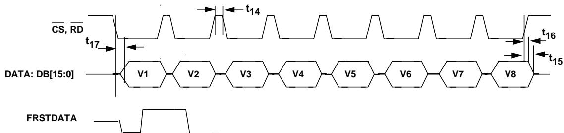
Figure 5. \overline{CS} and \overline{RD} linked Parallel Mode
