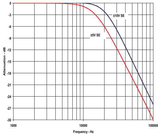
Figure 35 Analog Anti-Alias Filter Frequency Response
