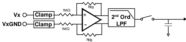
Figure 32 Analog Input Circuitry
